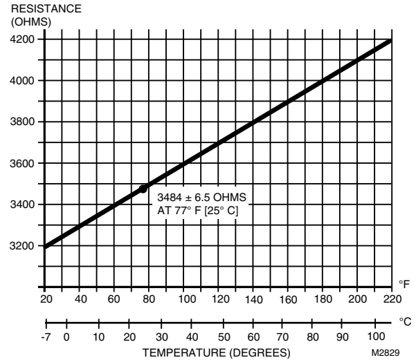
Fig. 7—Resistance vs. temperature performance characteristics.
